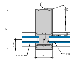
② VERTICAL VISION DETAIL 6" = 1'-0"
