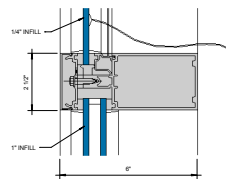
③ HORIZONTAL SPANDREL DETAIL 6" = 1'-0"
