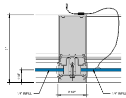
① VERTICAL SPANDREL DETAIL 6" = 1'-0"
