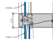
④ HORIZONTAL VISION DETAIL 6" = 1'-0"
